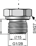
CG1/2 type G1/2" with flush diaphragm
