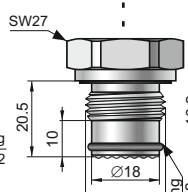
G1/2 type G1/2", Ø4 hole M type M20x1.5, Ø4 hole
